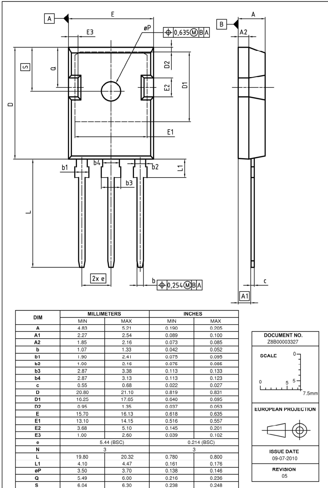
Figure 1 Outline PG-TO 247-3, dimensions in mm/inches
